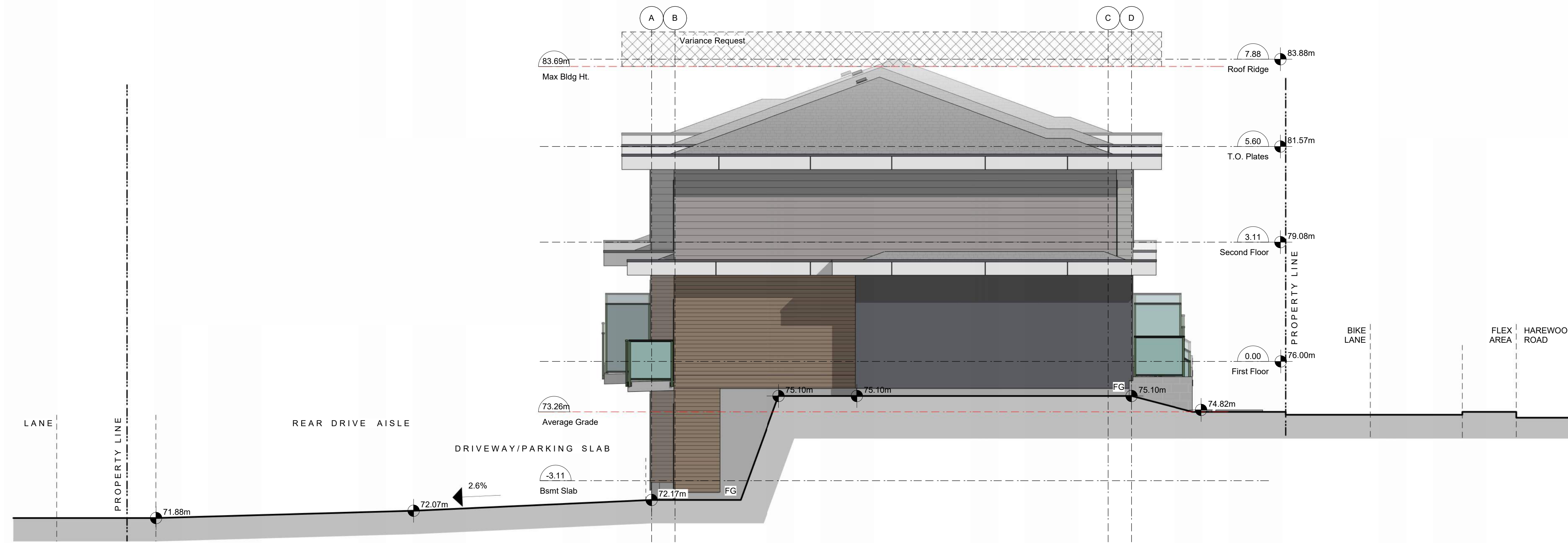
1 LEFT SIDE ELEVATION A303
